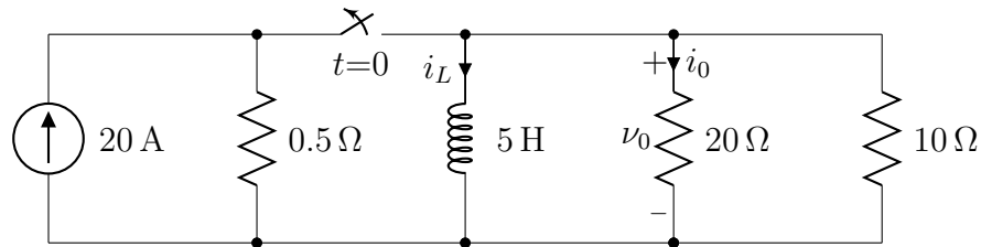
Figure 4.1: Einföld RL rafrás.
